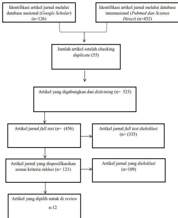
Gambar 1. Diagram PRISMA
